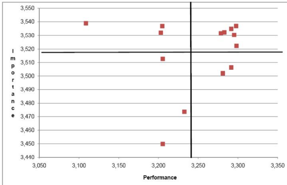
Gambar 3. I-P Analysis
