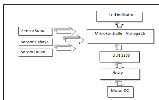
Gambar 2. Blok Diagram
