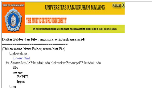
Gambar 7 Proses Import
